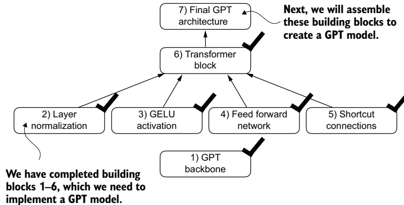
Figure 4.14 The building blocks necessary to build the GPT architecture. The black checks indicate the blocks we have completed.
